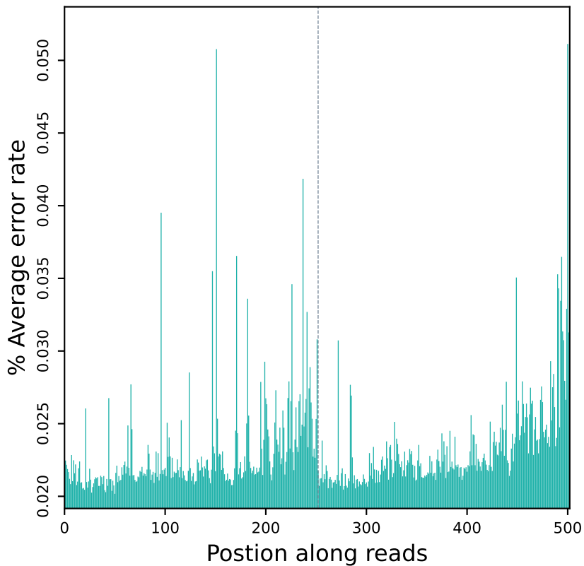
Error rate distribution along reads (R20201)
